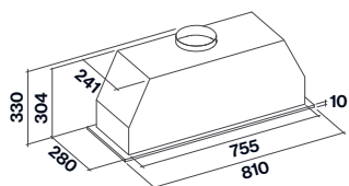
Cut-out size: 762 mm x 245 mm
