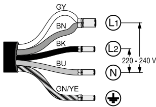
220-240V/380-415V 3N~
