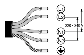
220-240V/380-415V 2L/2N~
