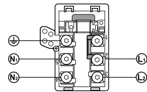
220-240V/380-415V 2L/2N~
